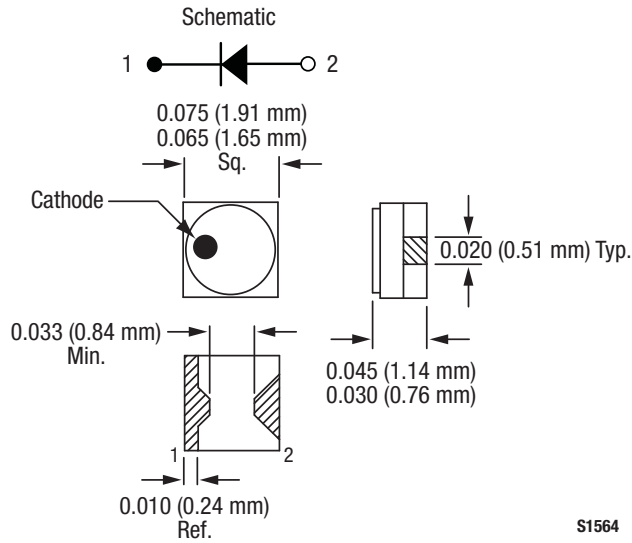
Figure 17. -219 Package
